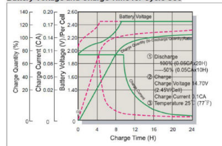
Charging Procedures
