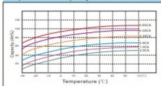
Constant current characteristics (A, 25°C)
