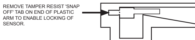
Figure 2: Tamper Resist Activation
