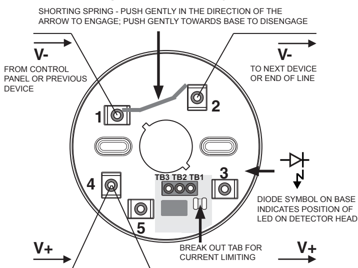
Figure 1: Terminal Layout
